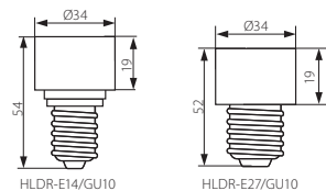
HLDR-E14/GU10
