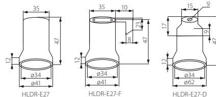
HLDR-E27
