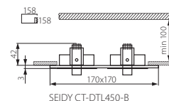
SEIDY CT-DTL450-B
