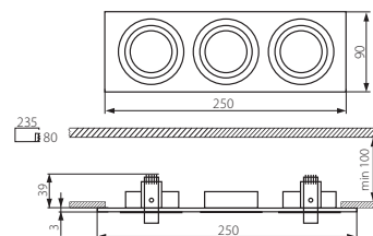
SEIDY CT-DTL350-B
