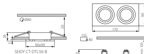
SEIDY CT-DTL50-B
